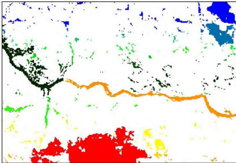
Figure 5.2: An example of the Connectivity Index Image for the Williams River Area.
