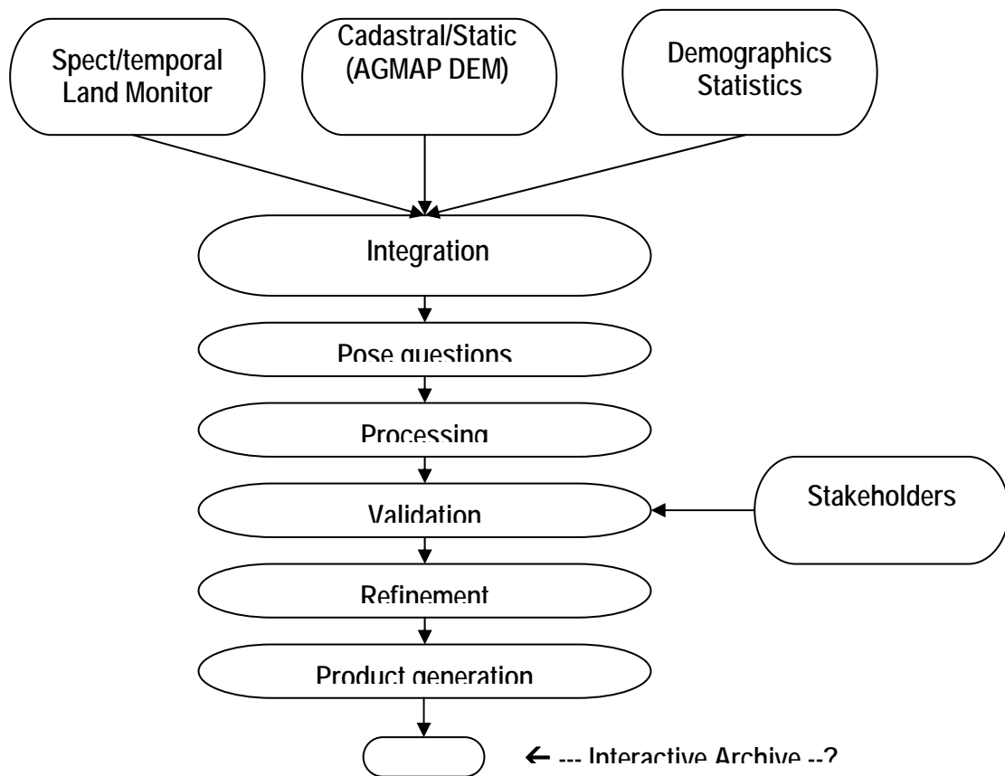
Figure 5.1: The data processing and validation model has for practical purposes been undertaken in three semi-iterative phases: accumulation, integration and validation.
